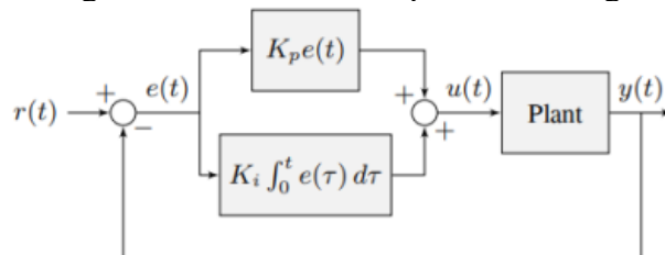
Gambar 12 Diagram Blok Kendali Proportional-Integral
