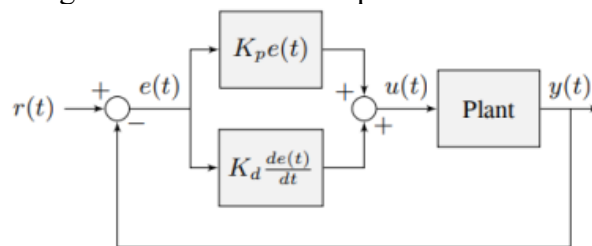
Gambar 13 Diagram Blok Kendali Proportional-Derivative
